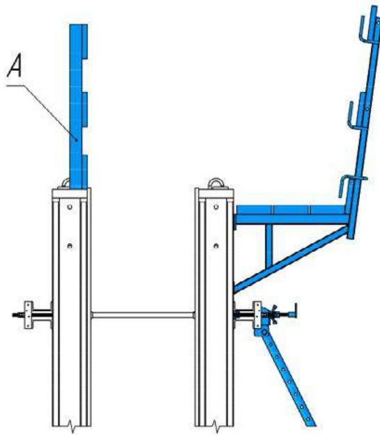
(A) Opposing guard-rail (provided at site)
