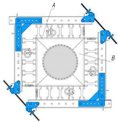
Circular column formwork
